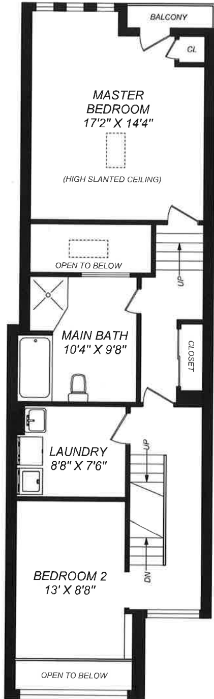
SECOND FLOOR 817 SQUARE FEET (CEILING HEIGHT : 8'-0")
