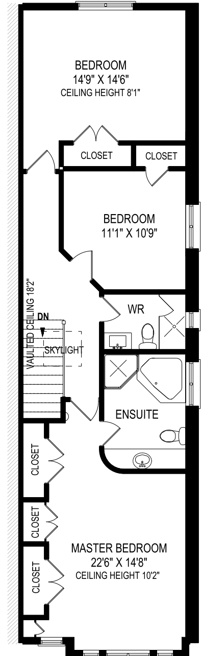
SECOND FLOOR 961 SQUARE FEET
